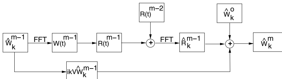
Fig. 2. Complete dataflow diagram of the time-stepping method.
