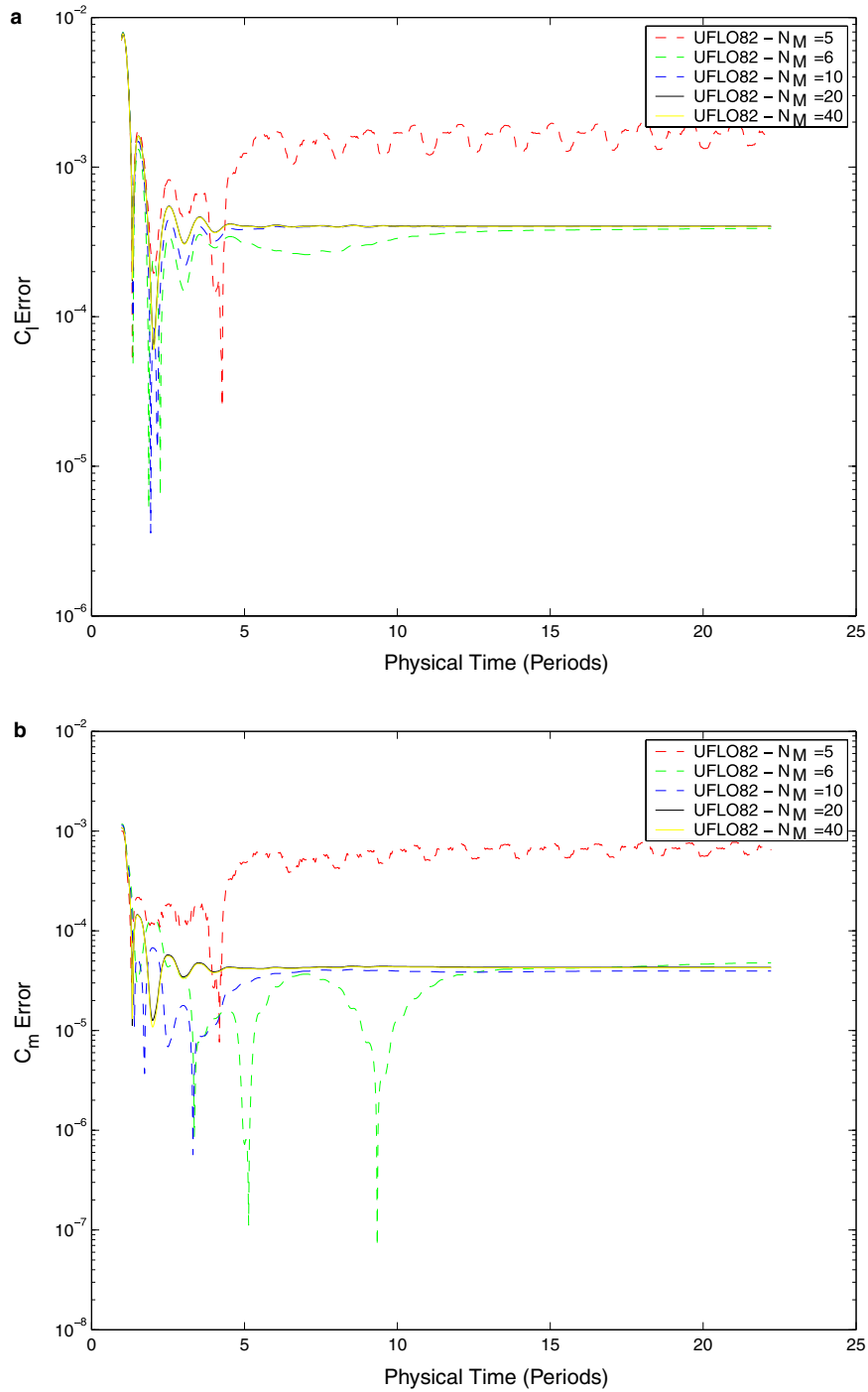
Fig. 11. Error as a function of physical time in units of periods for the UFLO82 solution calculated with 45 time steps per period: (a) lift and (b) moment.
